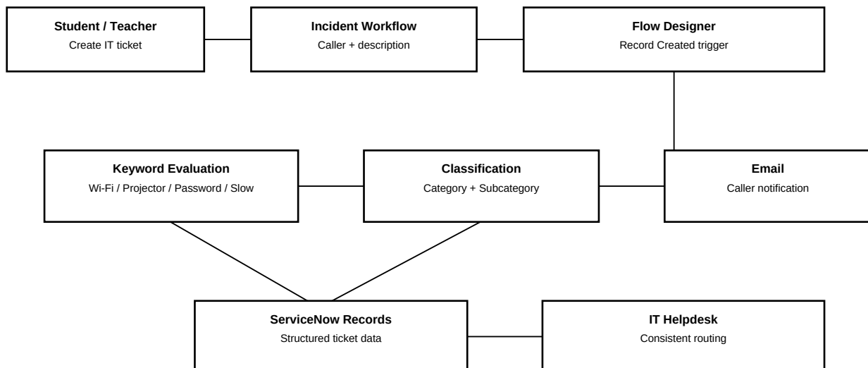
Figure 1: Architecture and data flow of the Auto Ticket Classification solution
